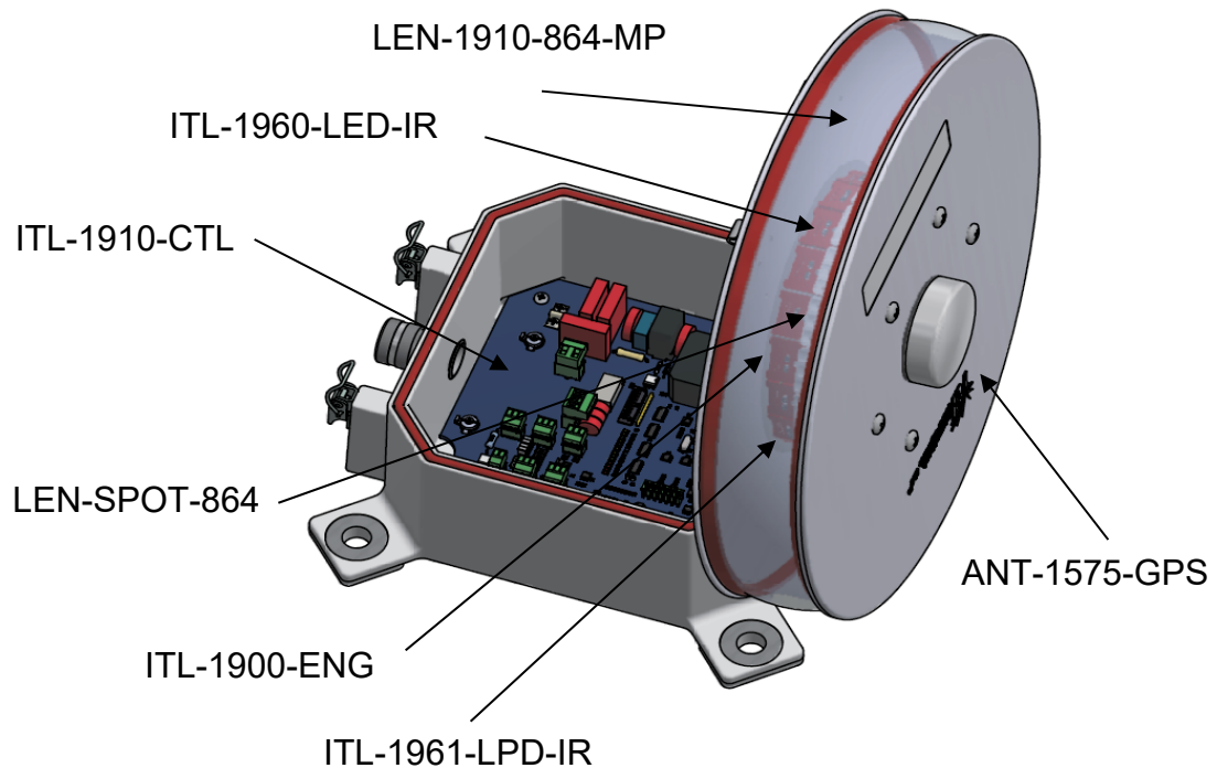
Figure 13: IFH-1910-0IR Replacement Parts Detail
