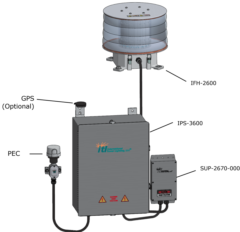
Figure 1: ILS-2600 White LED System
