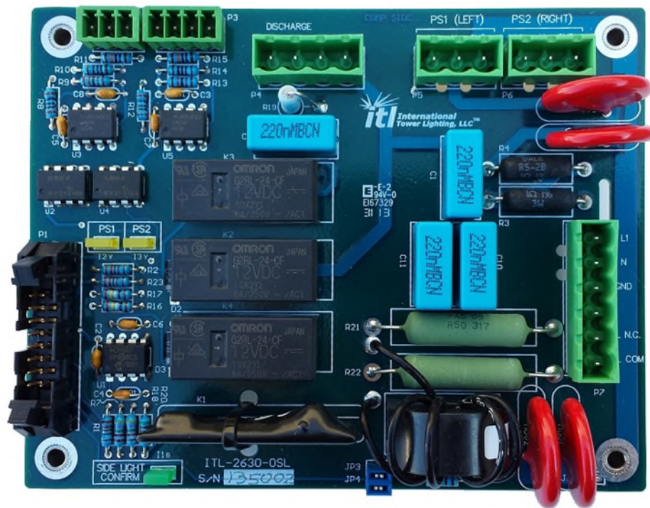
Figure 44: ITL-2630-OSL Side Light Board
