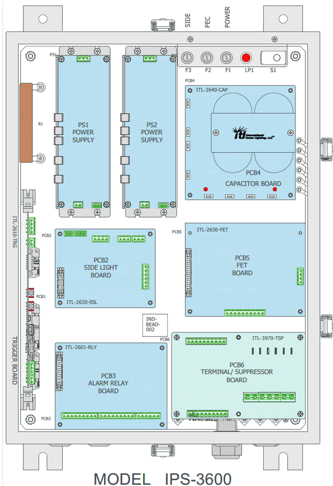
Figure 15: IPS-3600 Power Supply Panel Component Locator
