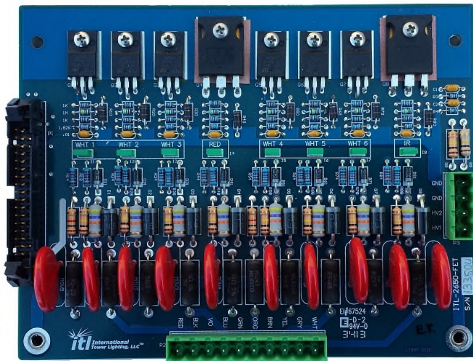
Figure 43: ITL-2650-FET Driver Board
