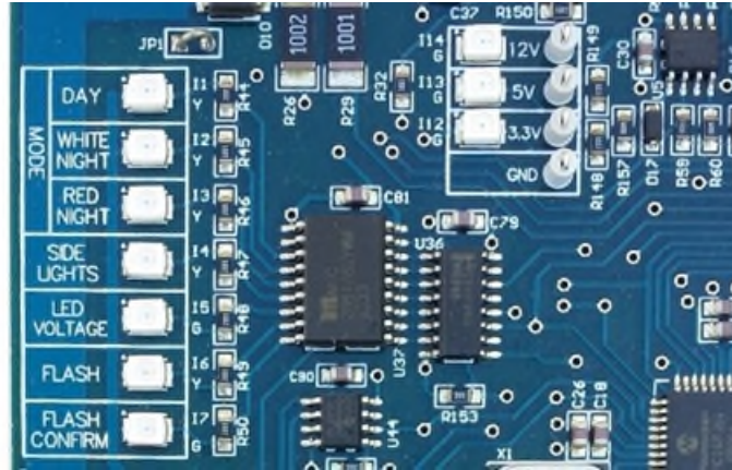
Figure 37: ITL-2610-TRG LED Location Detail
