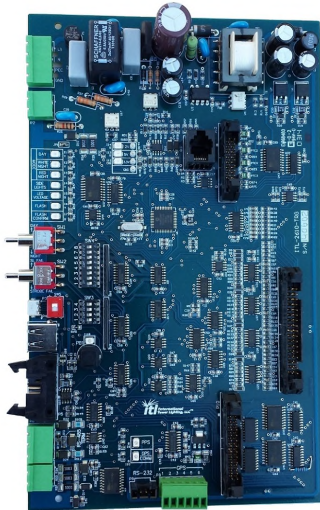
Figure 36: ITL-2610-TRG Trigger Board
