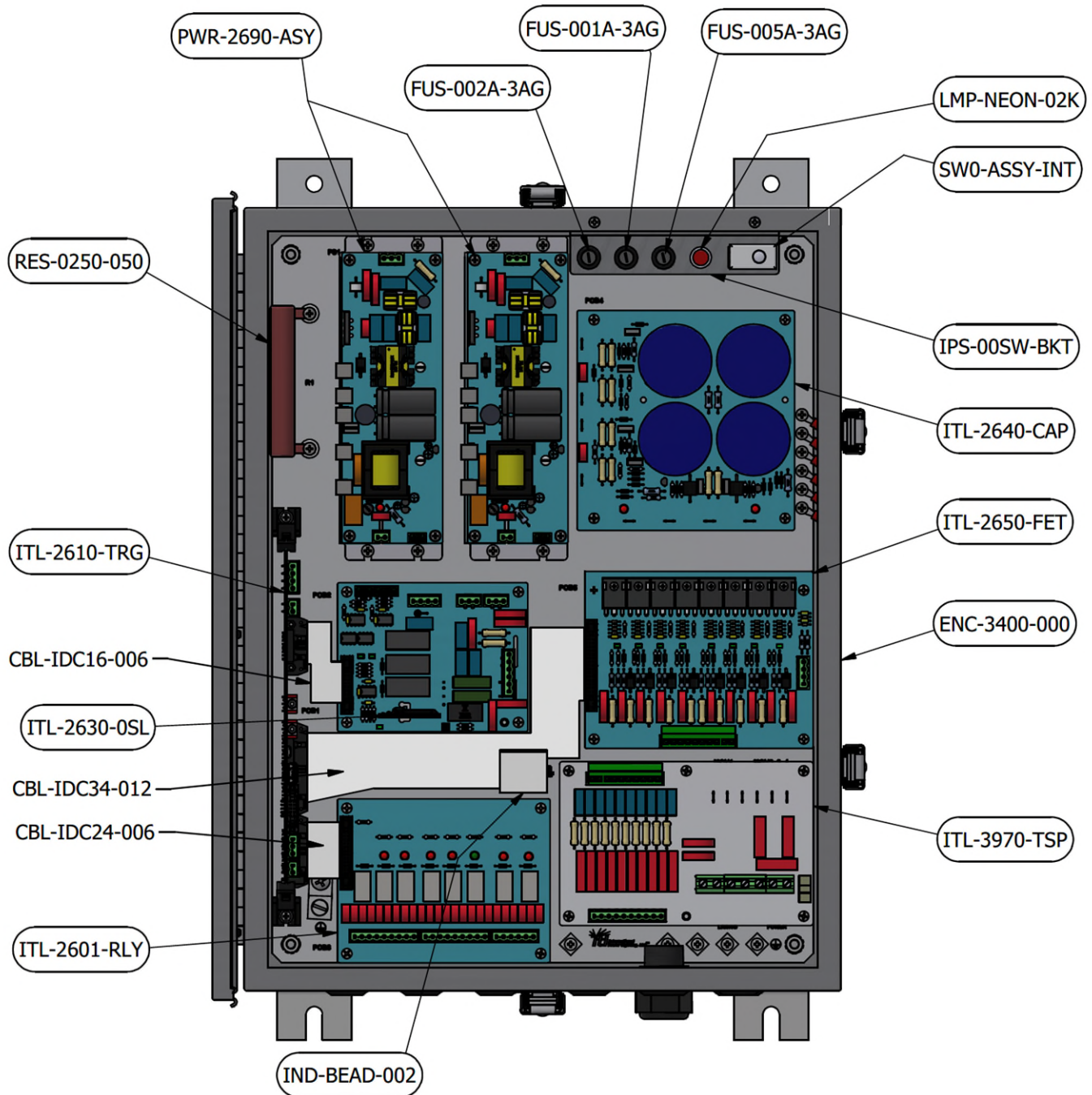
Figure 13: IPS-3600 Power Overall Component Layout
