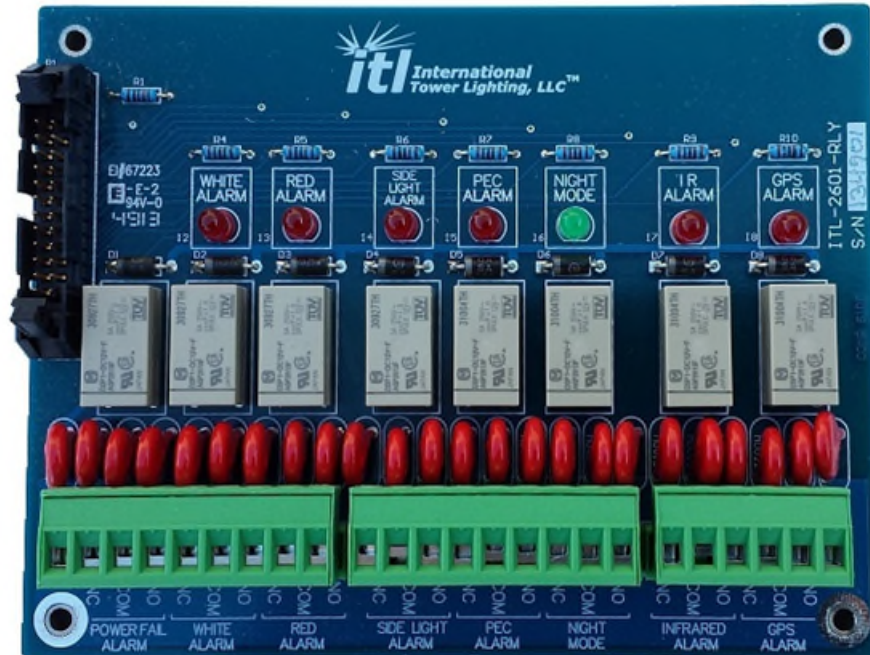
Figure 45: ITL-2601-RLY Alarm Relay Board
