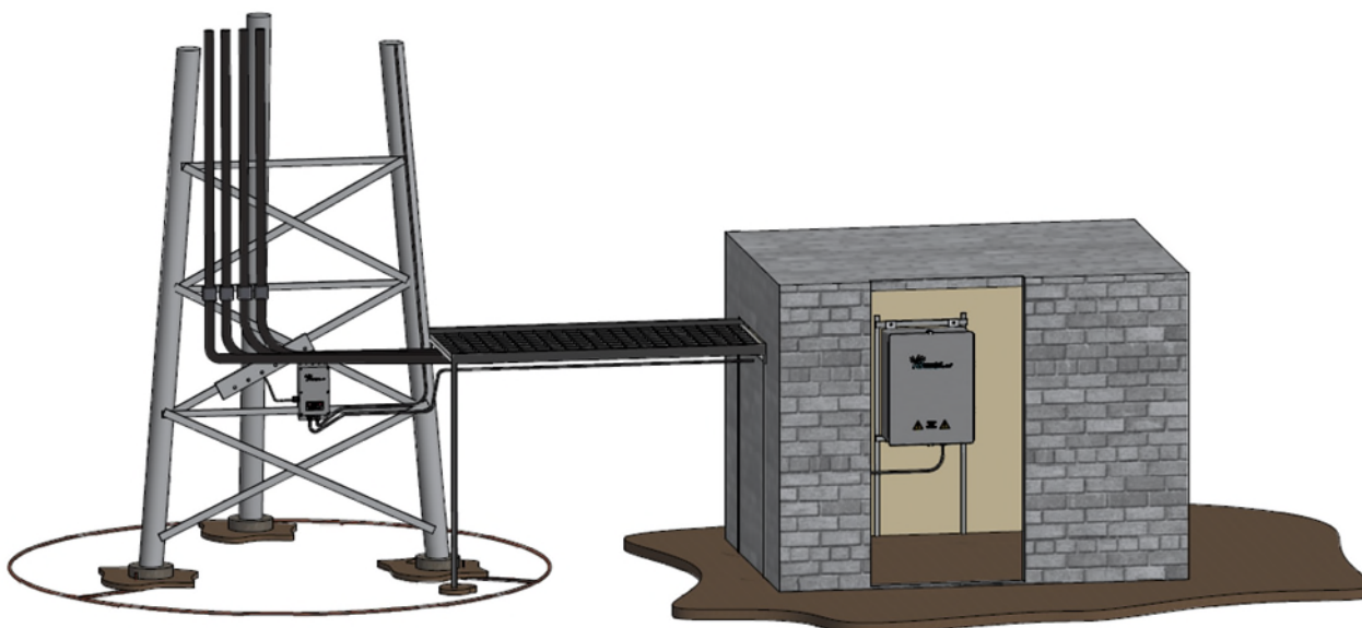
Figure 10: Above Ground Flash Head Cable Suppressor Installation
