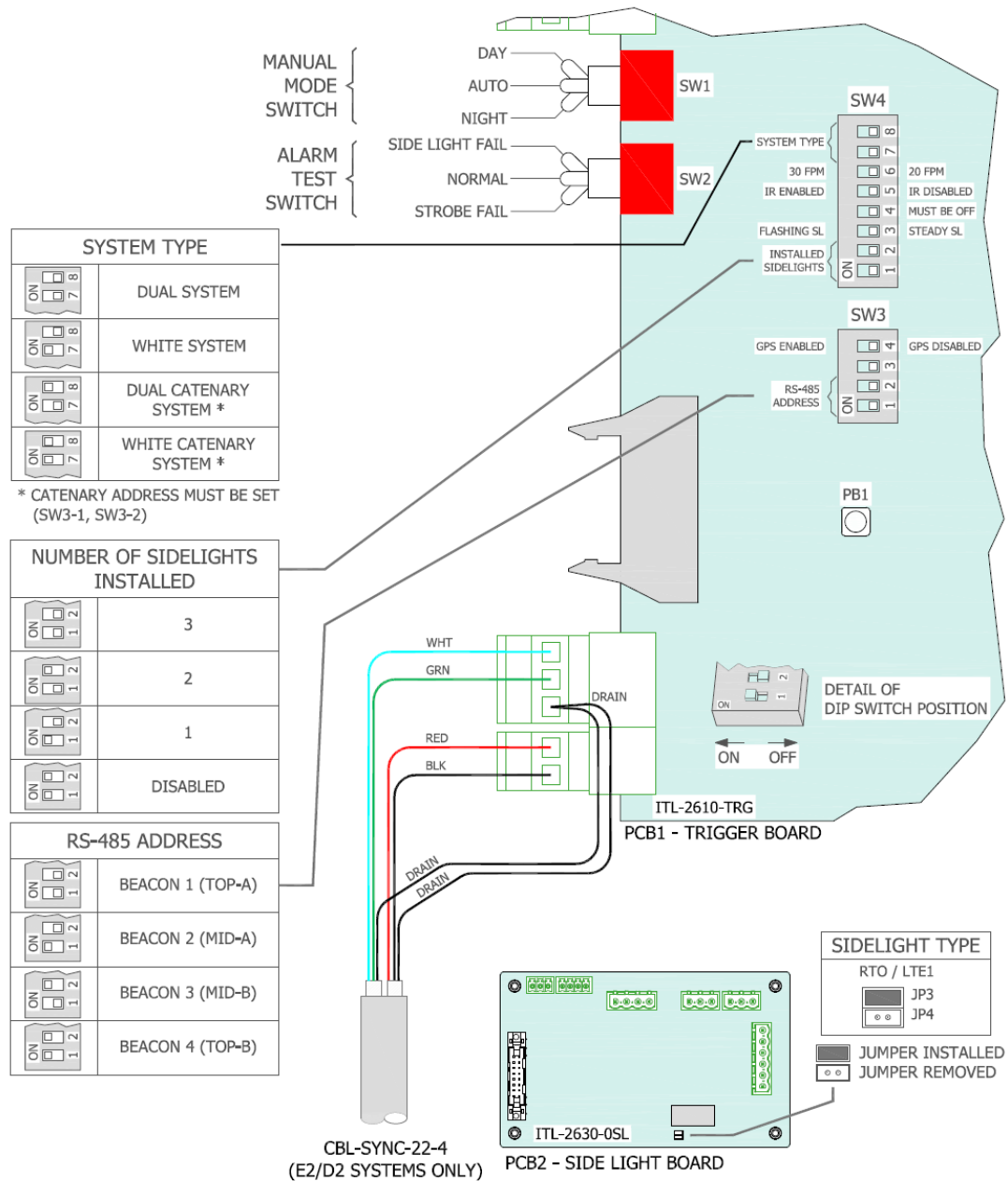
Figure 40: ITL-2610-TRG Switch Settings
